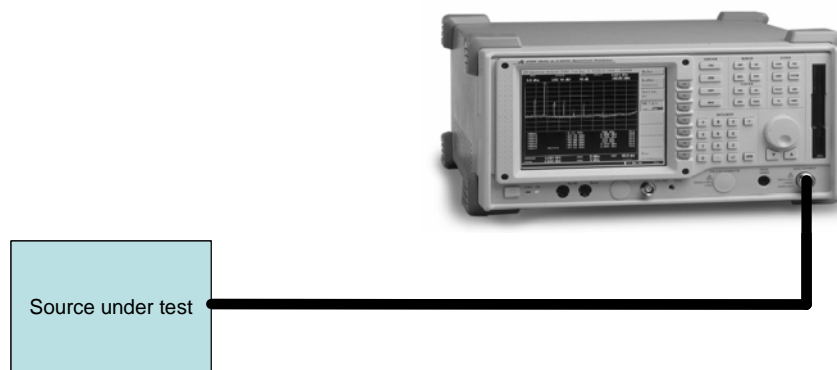
Figure 7: Phase noise measurement with a spectrum analyzer
