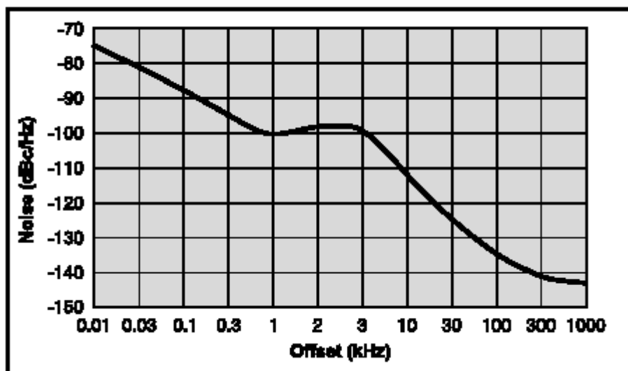
Figure 4: Phase noise of a low cost signal generator
